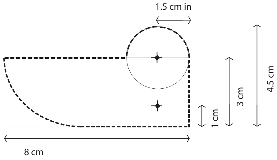
6. Bottom jaw
